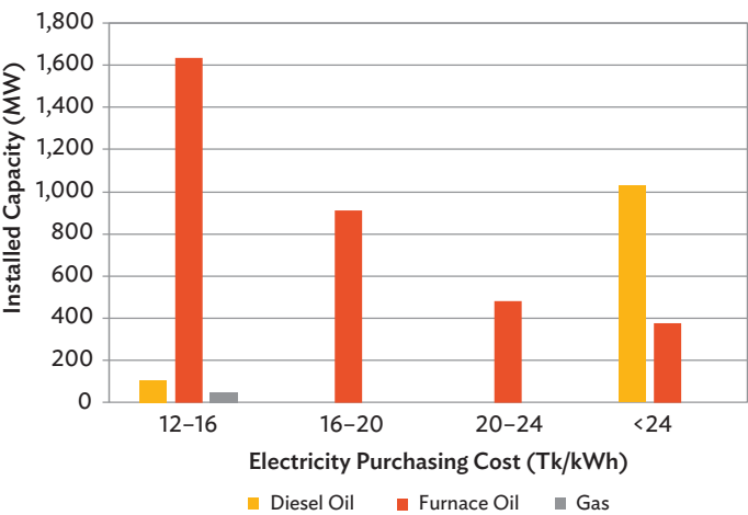
Figure 7: Generation Capacity of Power Plants with Expensive Purchasing Costs, July 2019–June 2020
